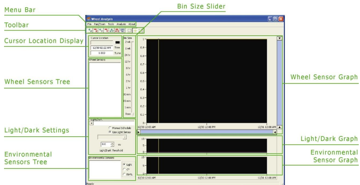
Figure 1-1 - Main Screen Labeled
